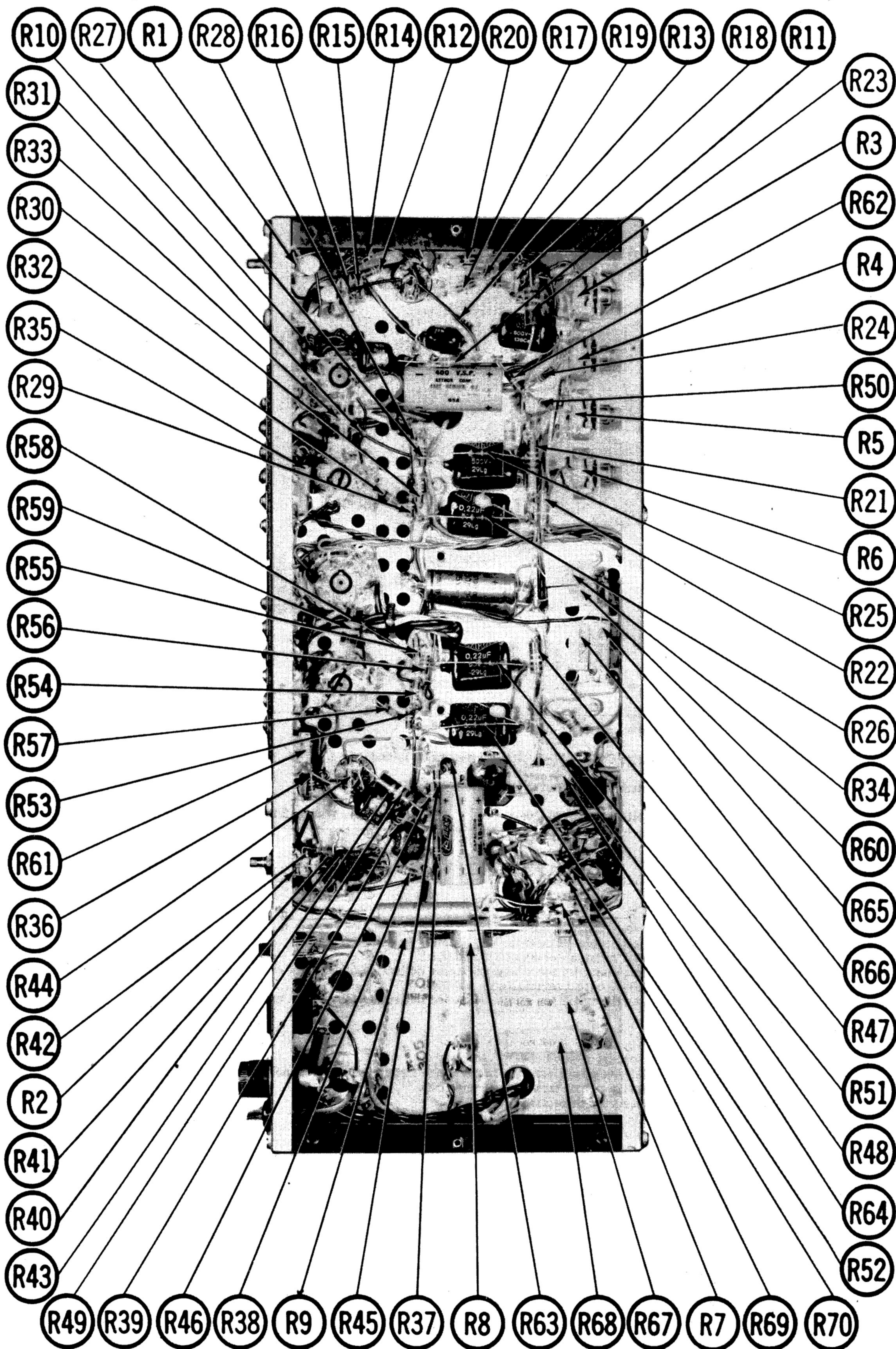
CHASSIS BOTTOM VIEW-RESISTOR IDENTIFICATION
