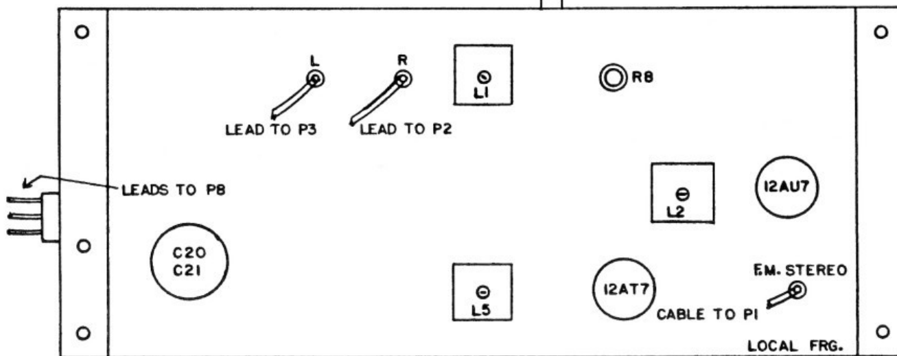
SA-510 TOP VIEW
