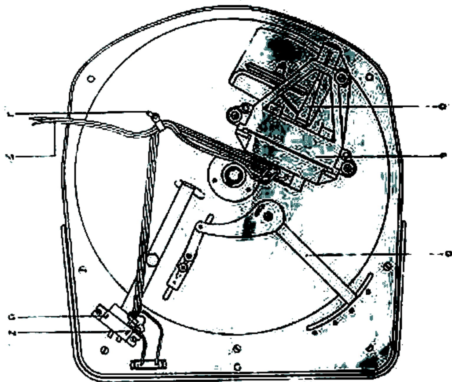
UNDERSIDE PLAN.
