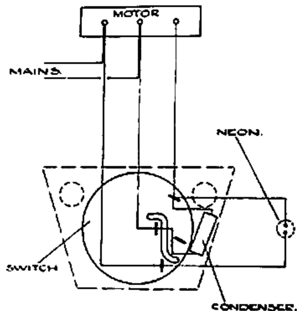
Wiring Diagram
