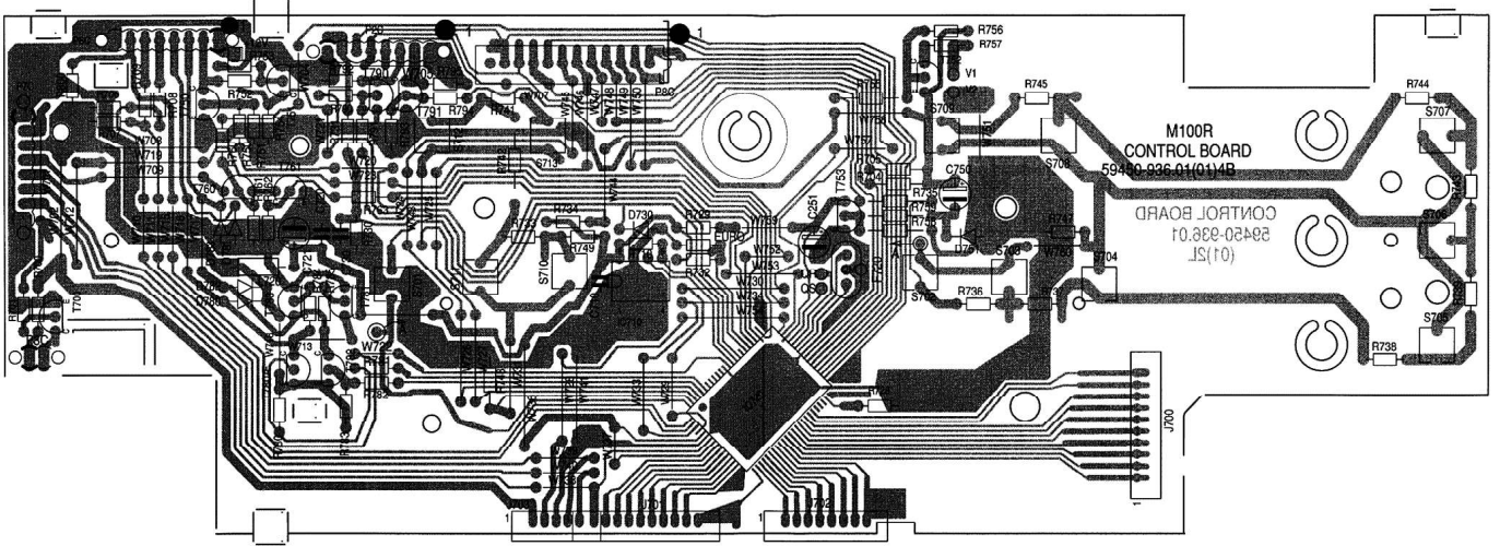
Bedienplatte / Control Board
