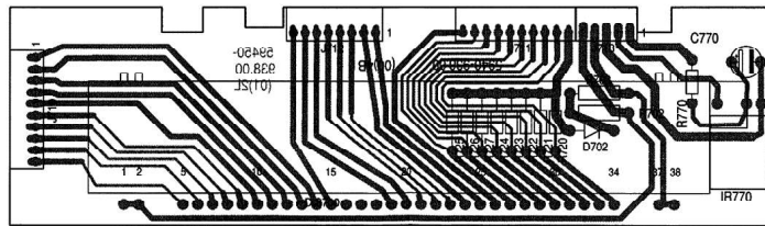
Displayplatte / Display Board
