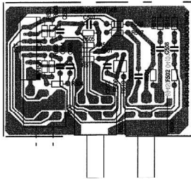
Klangreglerplatte / Tone Control Board
