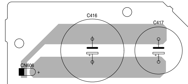
Eikoplatte / El. cap. PCB
