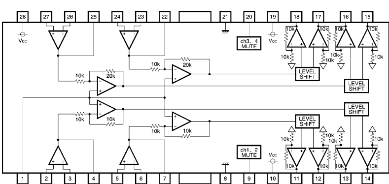
IC702 - BA5970FP
