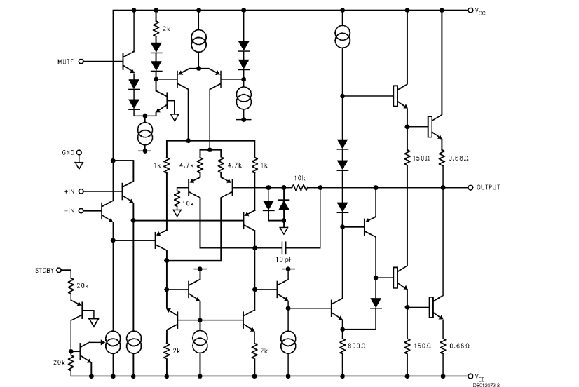
IC201 - LM1876T
