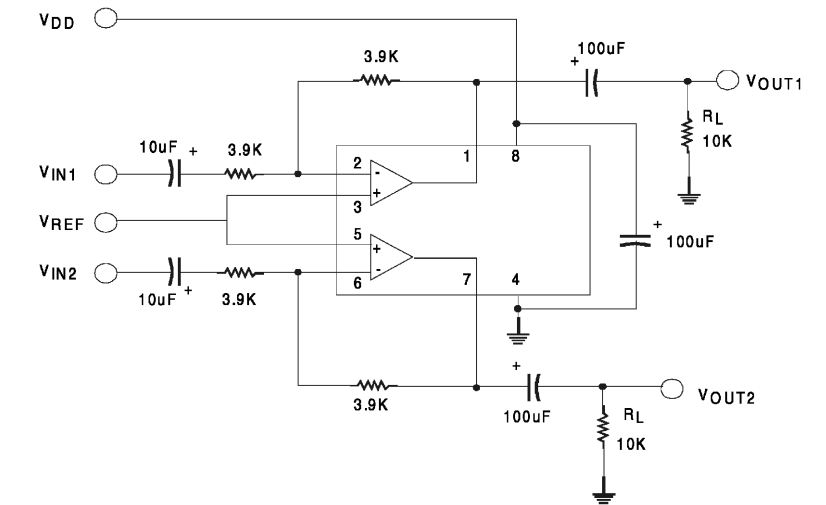
IC201 - LM1876T
