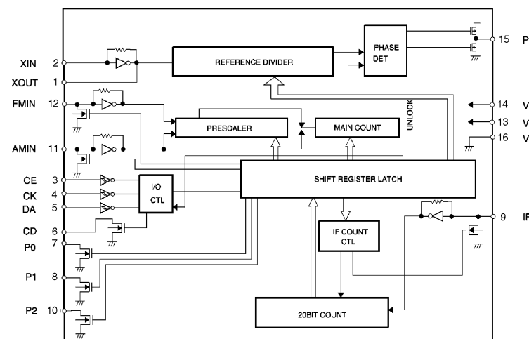
IC503 - BU2614FS
