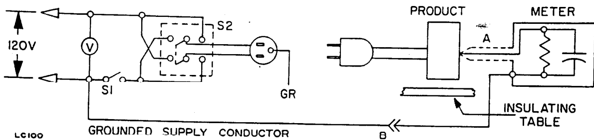
LEAKAGE CURRENT MEASUREMENT CIRCUITS
