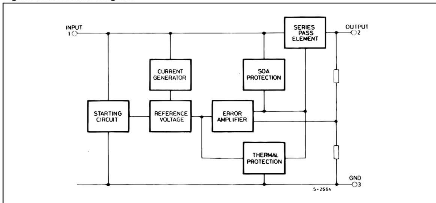
Figure 1: Schematic Diagram
