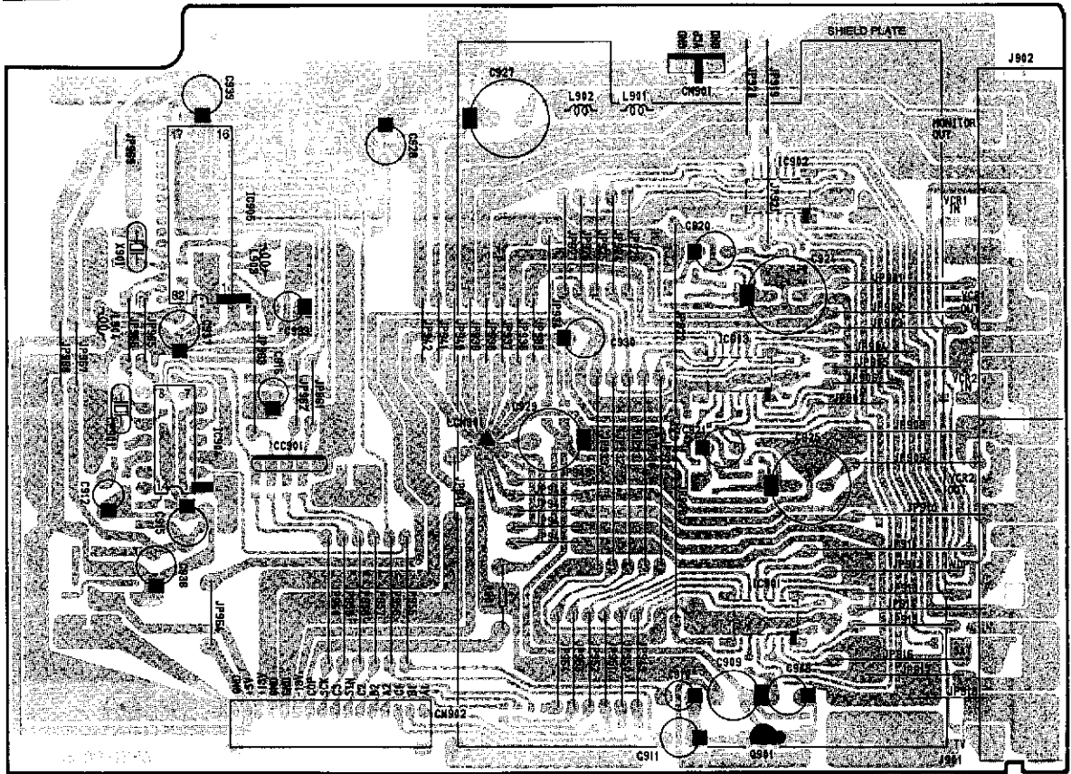
PCB-24 Video/On Screen P. C. Board (Parts Side)
