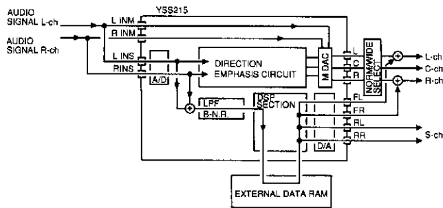
< Flow of signals within the system in the Dolby pro logic mode.
