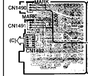
PCB-27 Line Out 2 P.C.Board
