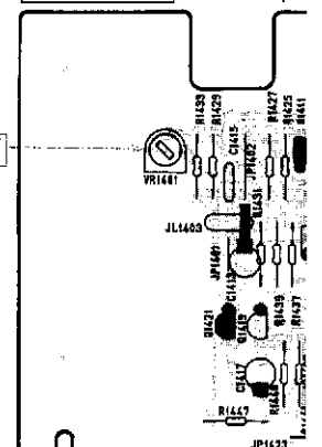
PCB-20 (2/2) PCB-21
