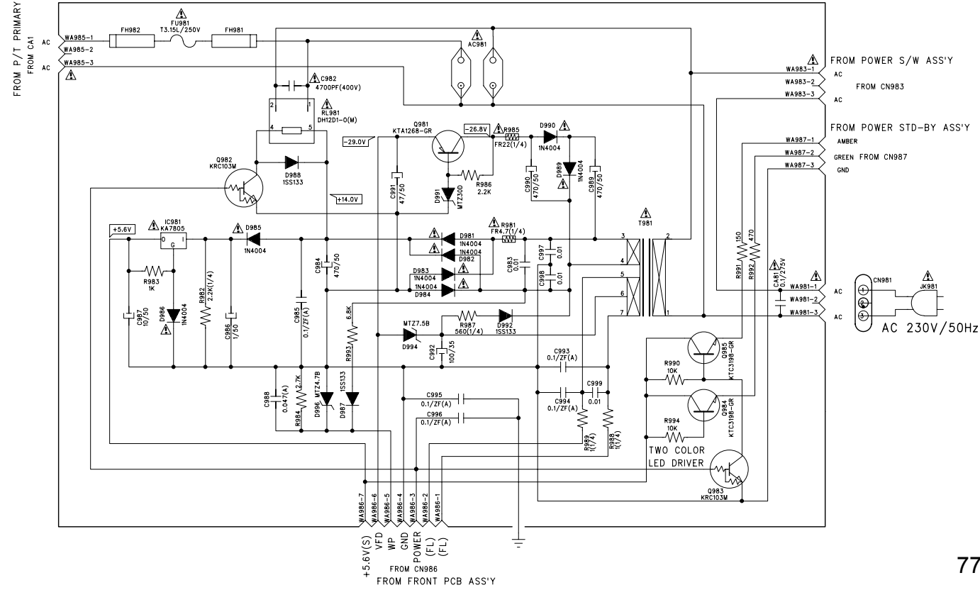
SUB POWER SUPPLY ASS'Y
