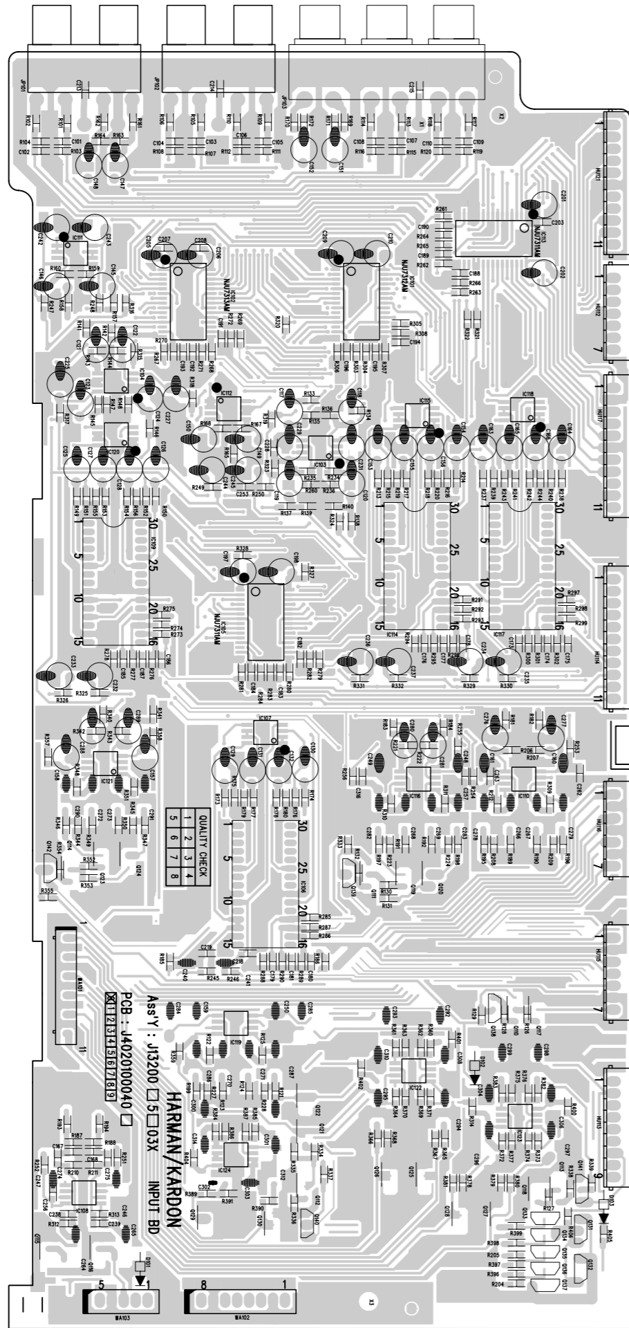
AUDIO P.C. BOARD (TOP VIEW)
