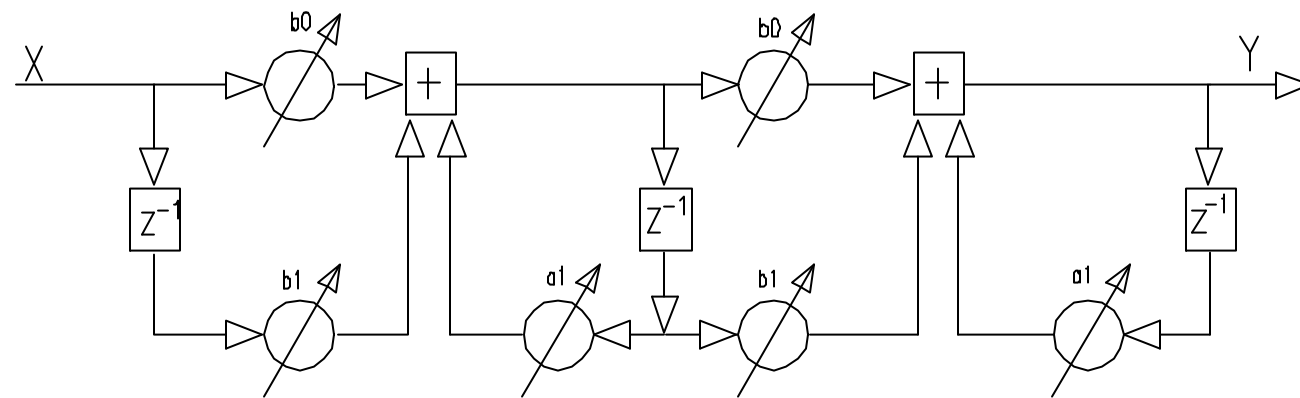
Fig 1-6 Filter Topology
