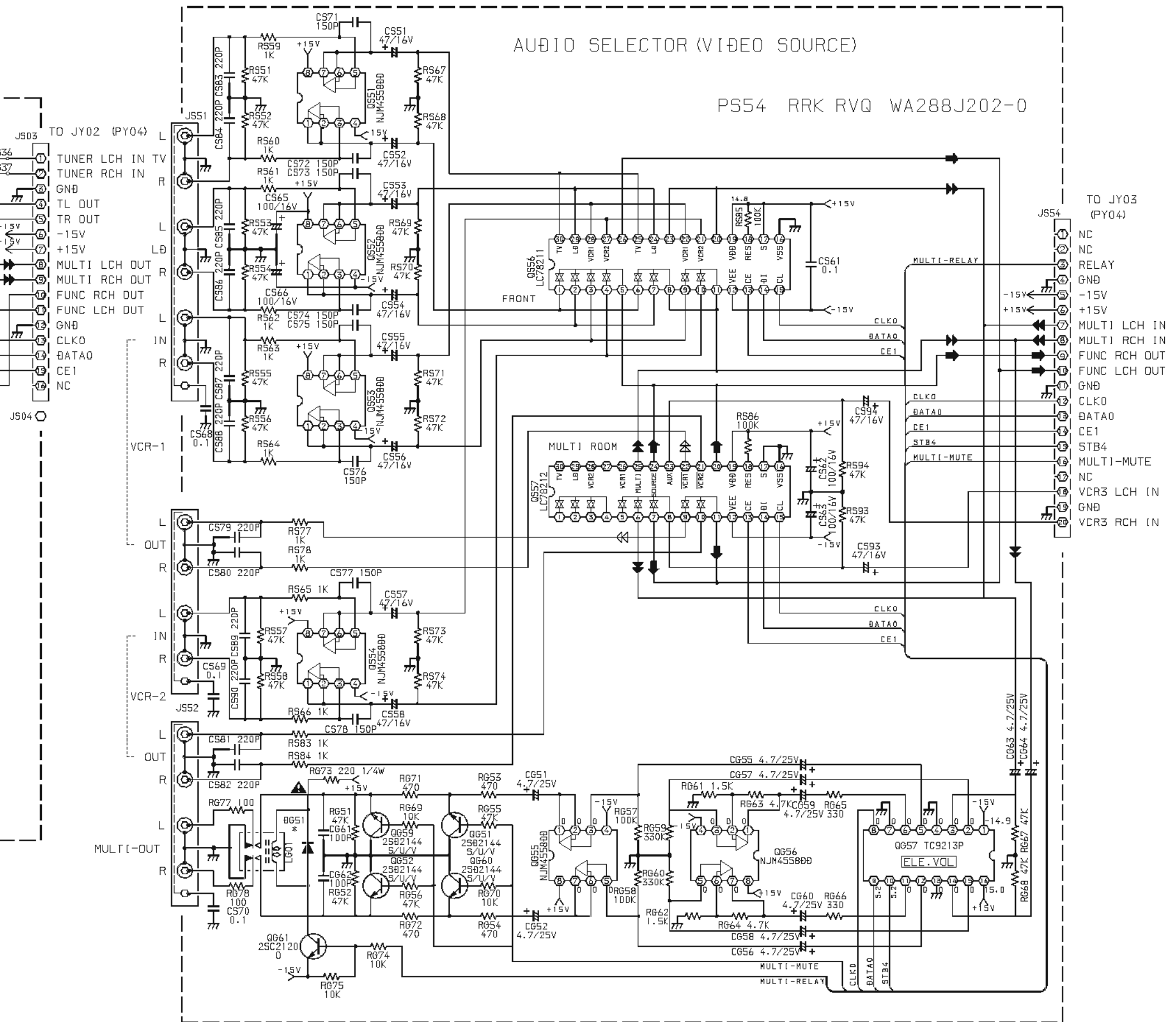
AVR85 European 230V Schematic 3 of 8
