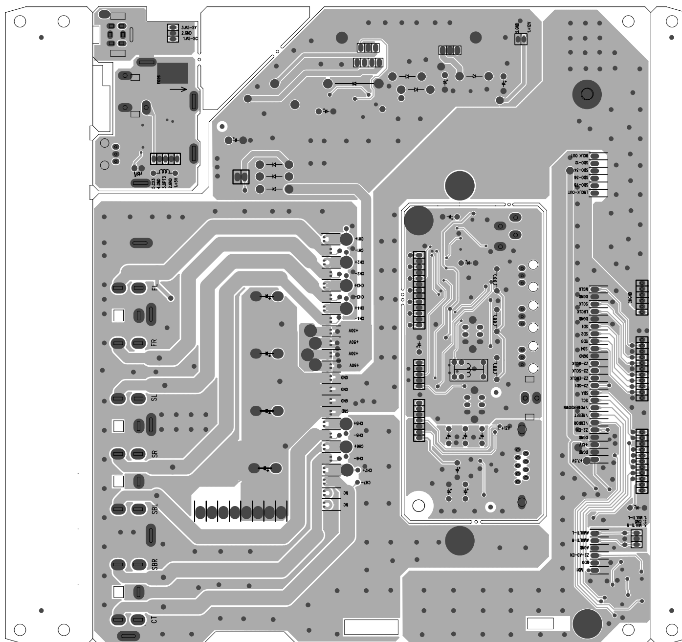
AMP BOARD (BOTTOM VIEW)
