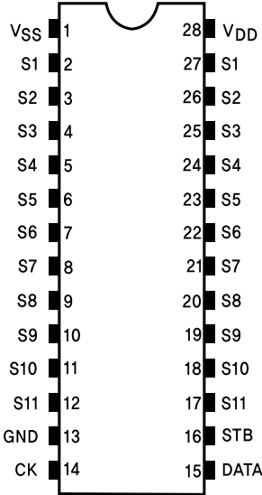
TC9273N, TC9273F
