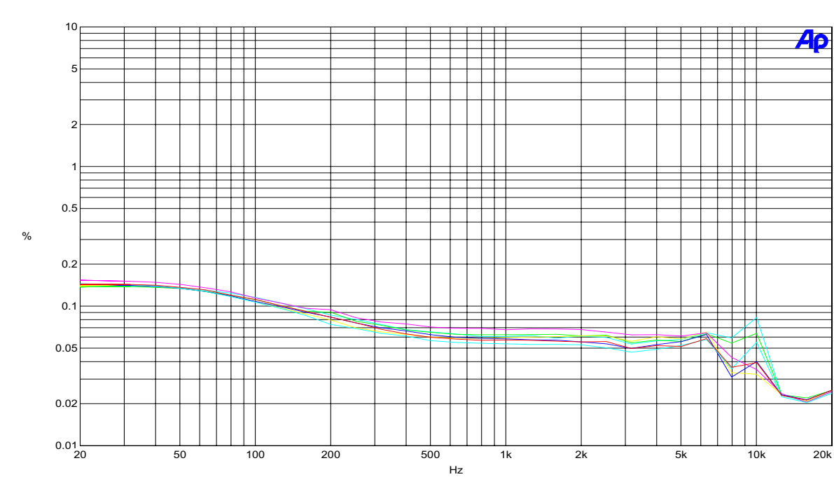
FIGURE 4: THD+N vs. Frequency
