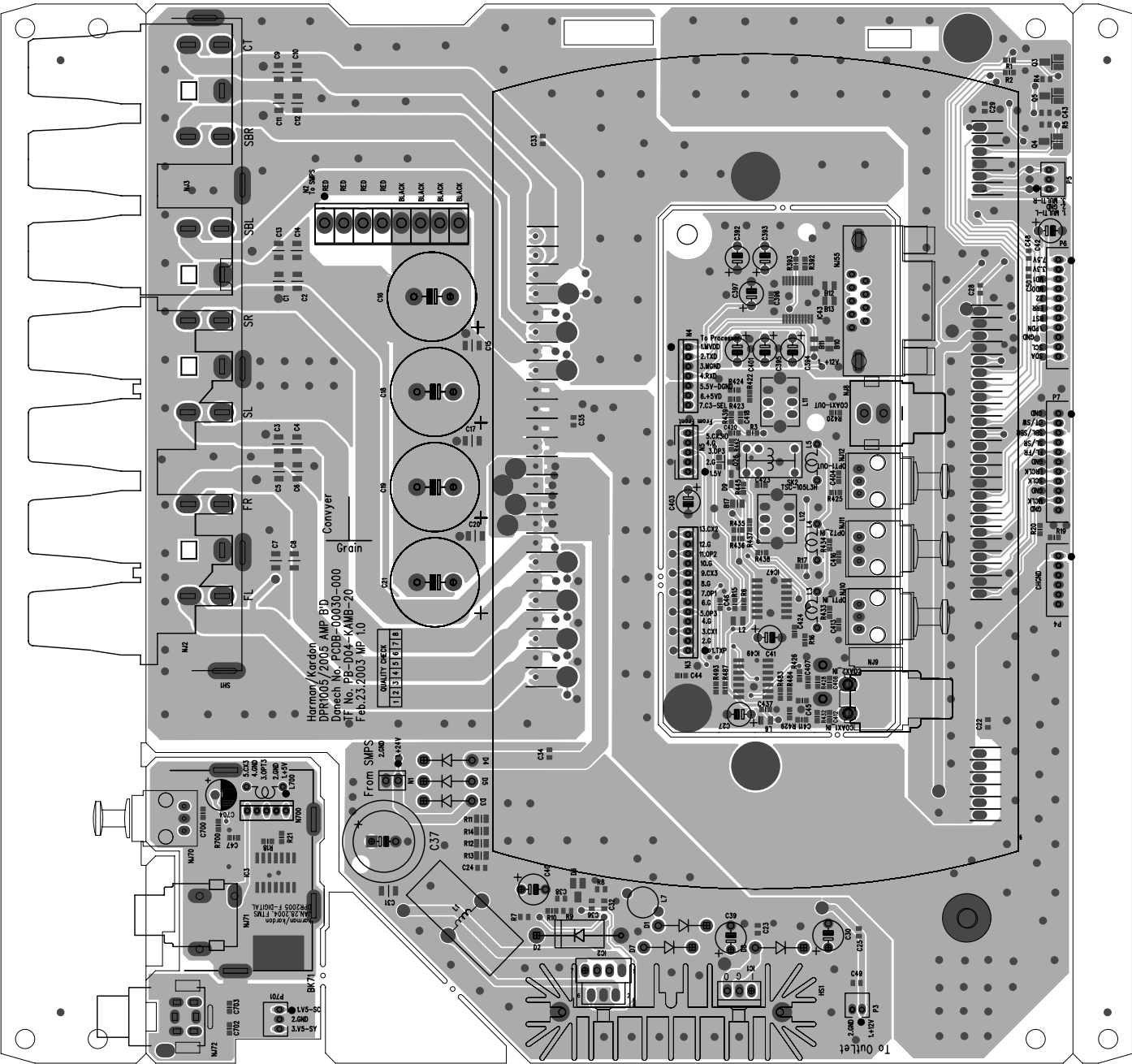
AMP BOARD (TOP VIEW)
