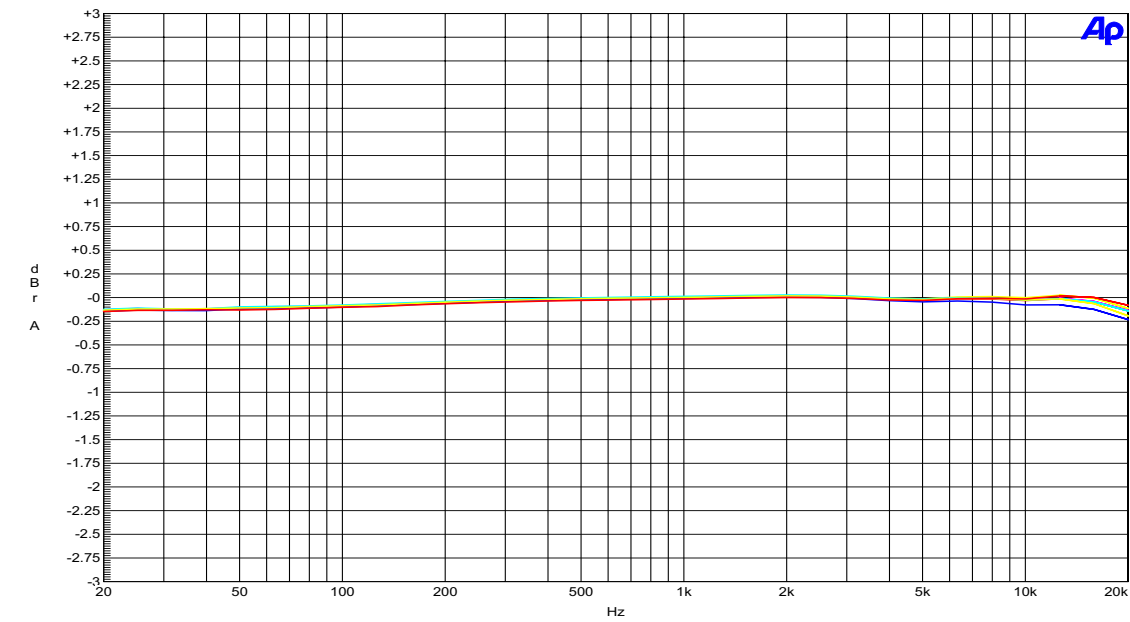
FIGURE 3: Frequency Response
