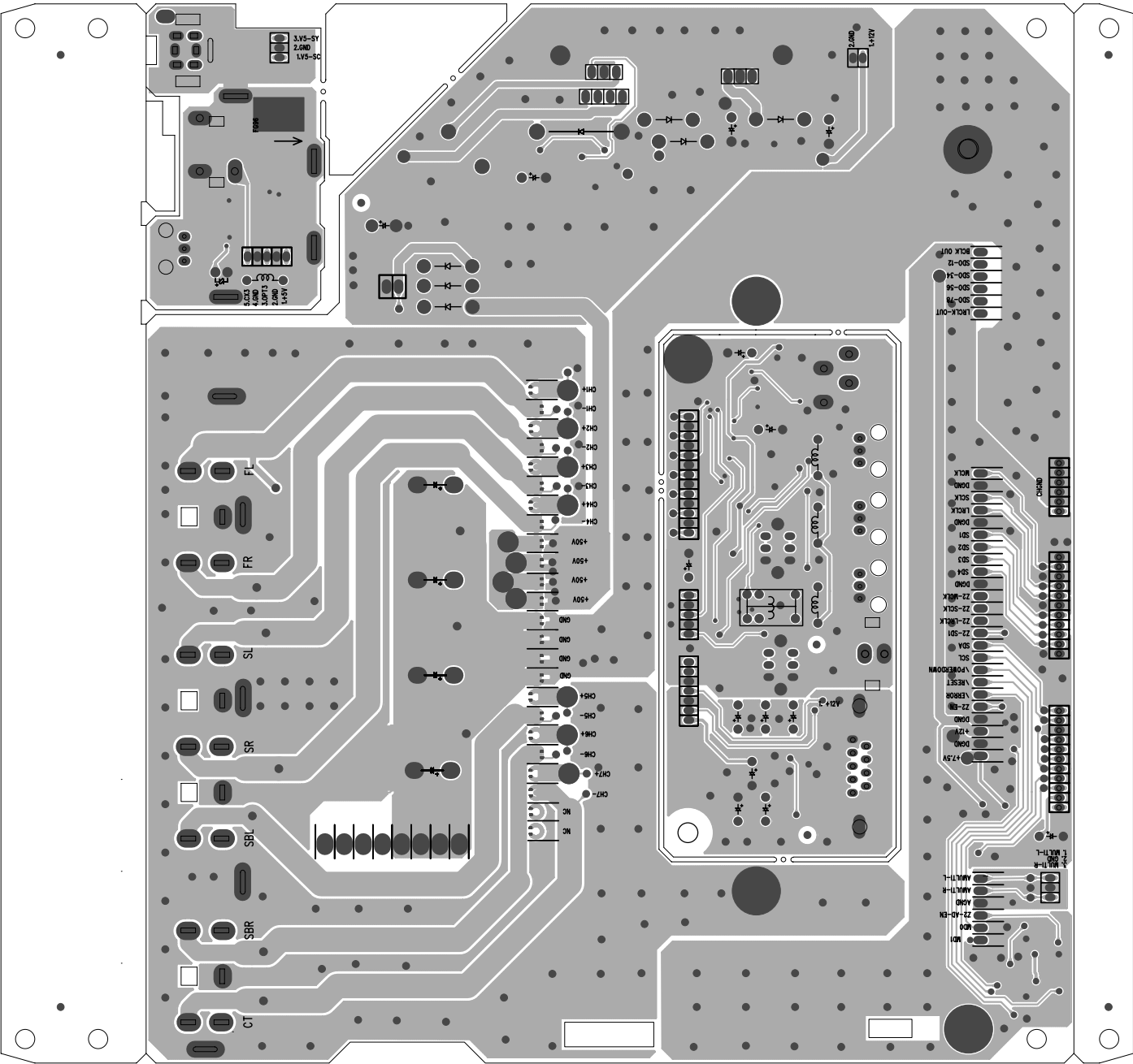
AMP BOARD (BOTTOM VIEW)
