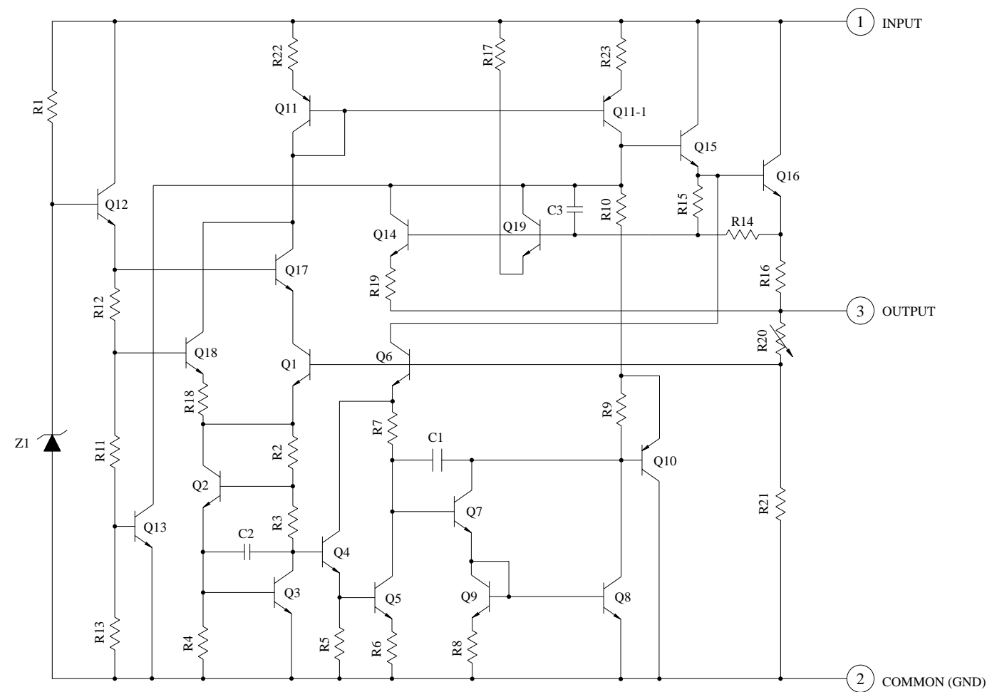
EQUIVALENT CIRCUIT
