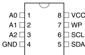
8-lead PDIP
