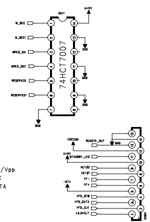
FRONT CONNECTOR
