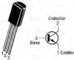
KRC107 PNP KTC3875S NPN KTA1504S PNP KRA107S PNP KTD1304 NPN 2N3904S NPN KRC 107S NPN 2SA1955 PNP
