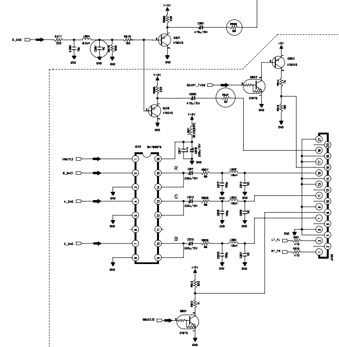
VIDEO OUT
