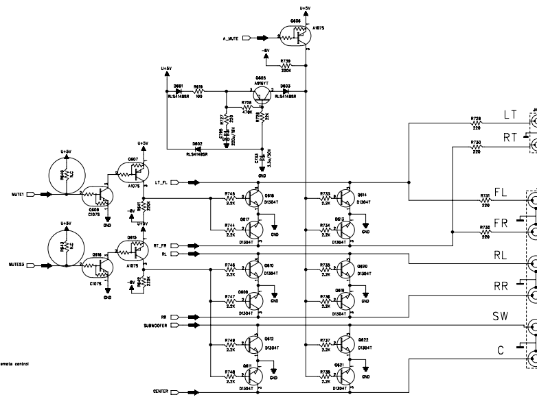
AUDIO OUT
