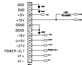
POWER PORT
