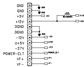
POWER PORT
