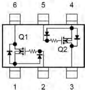
HN1K05FU N Channel
