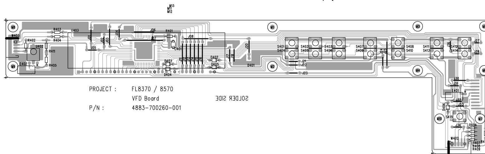
FL8370 VFD display board
