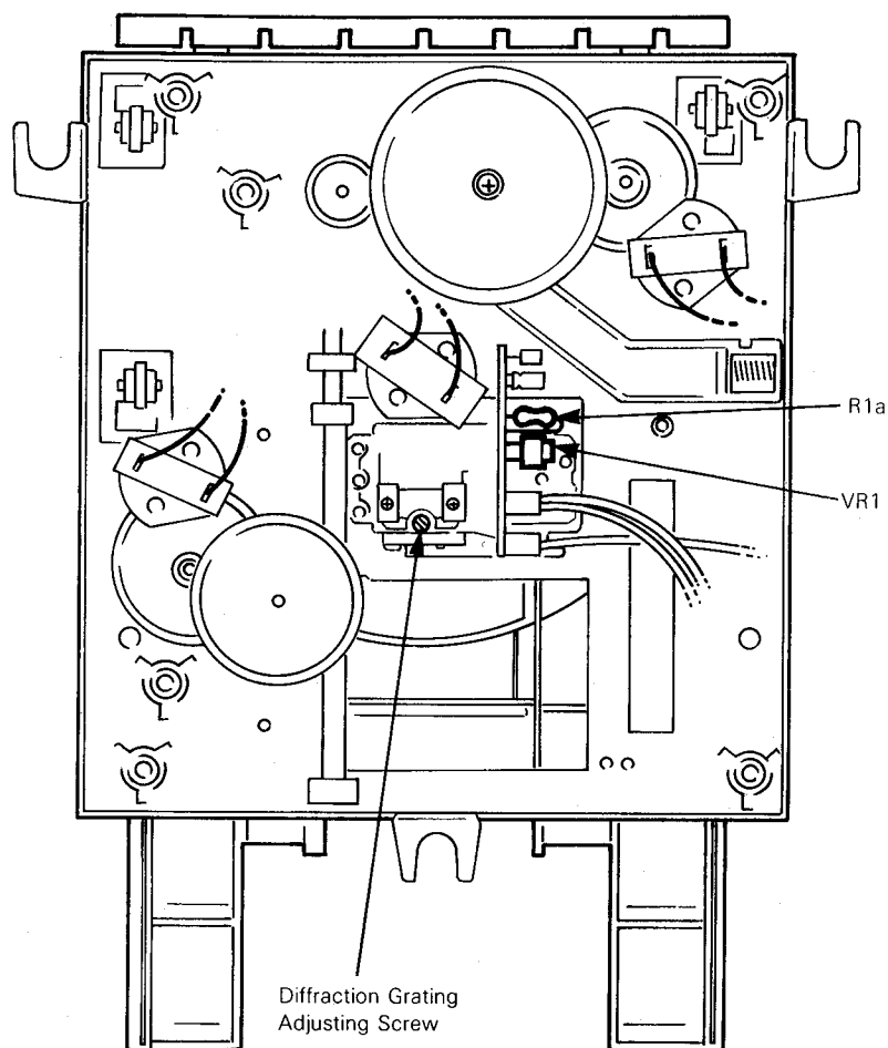
Bottom View
