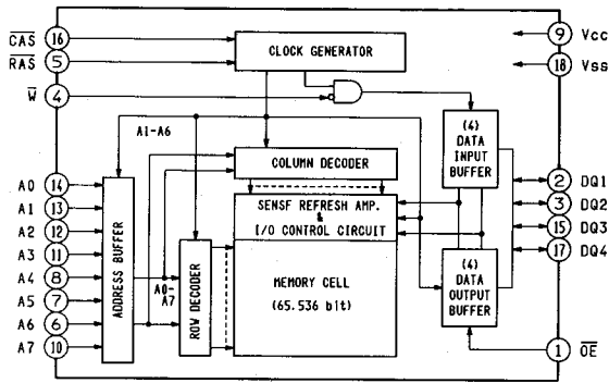
IC202 : M5M4416P 65536-Bit (16384-Word by 4-Bit) Dynamic RAM
