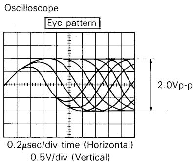
Waveforms 3T-11T
