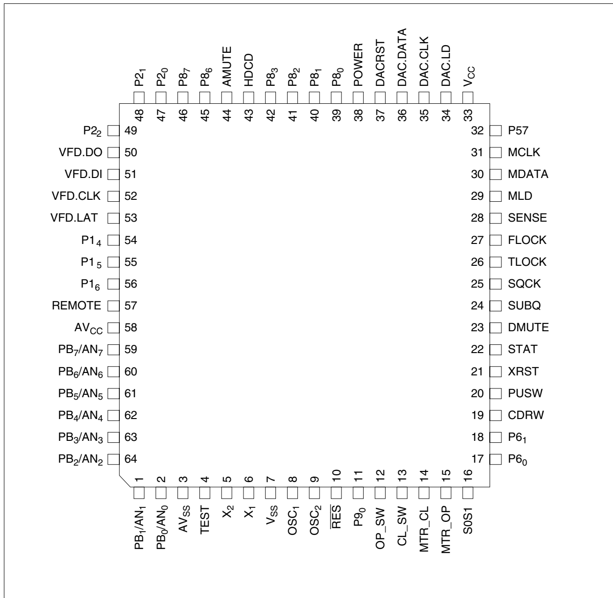
Figure 1.2 Pin Arrangement
