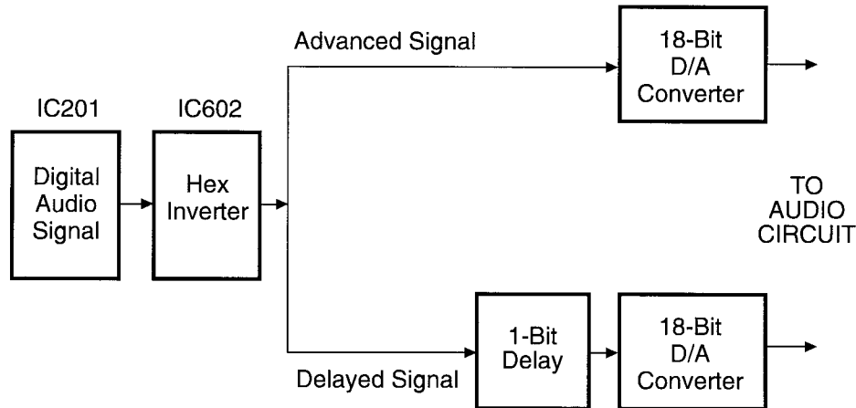
THE RLS SYSTEM (BLOCK DIAGRAM)
