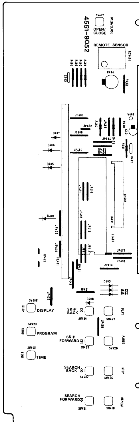
PCB-2 FRONT
