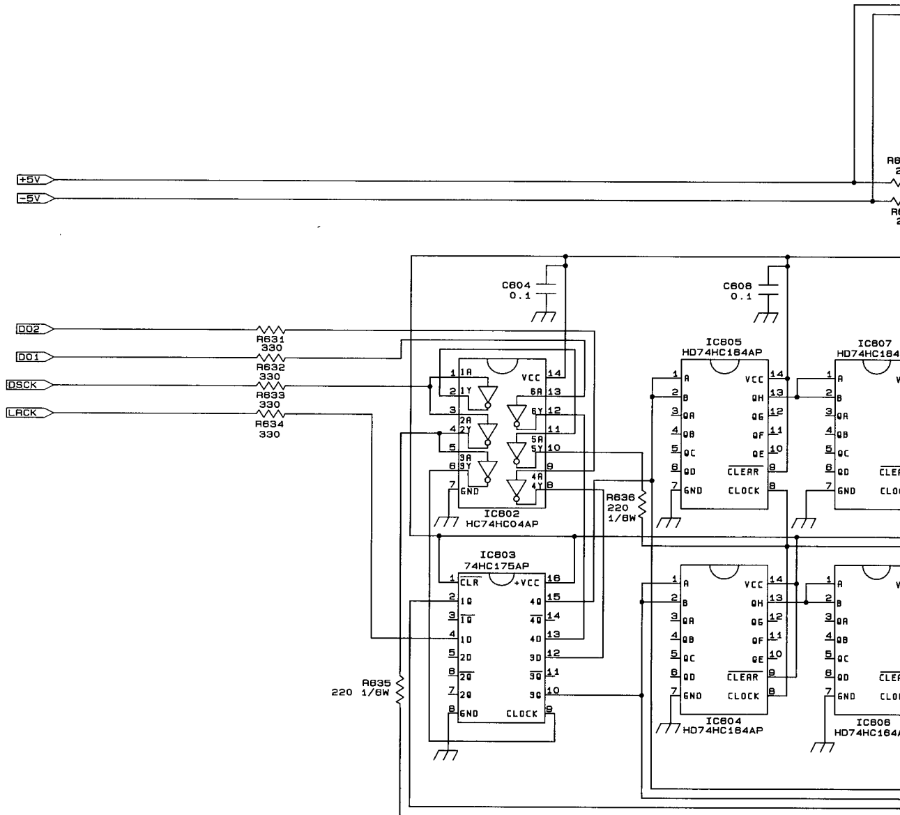
IC802
