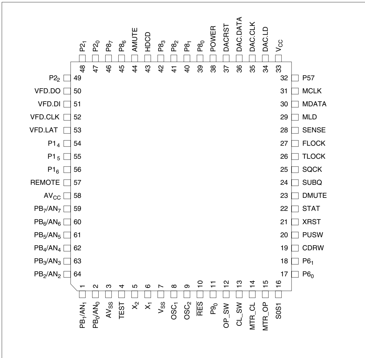
Figure 1.2 Pin Arrangement
