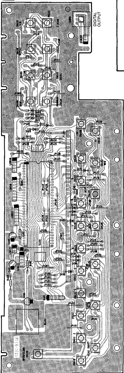
PCB-2 FRONT P. C. BOARD
