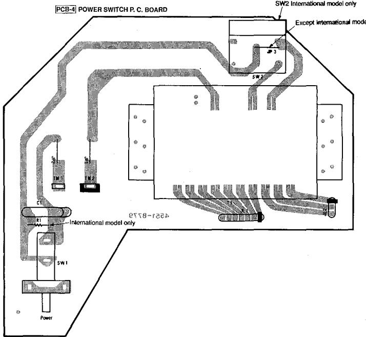
PCB-4 POWER SWITCH P. C. BOARD
