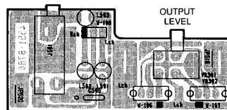
PCB-3 OUTPUT LEVEL & JACK P. C. BOARD HEADPHONES
