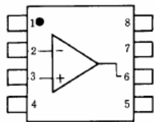
NJM5534M
