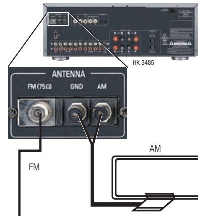
Figure 11 – Antenna Connections
