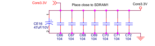
SDRAM1
