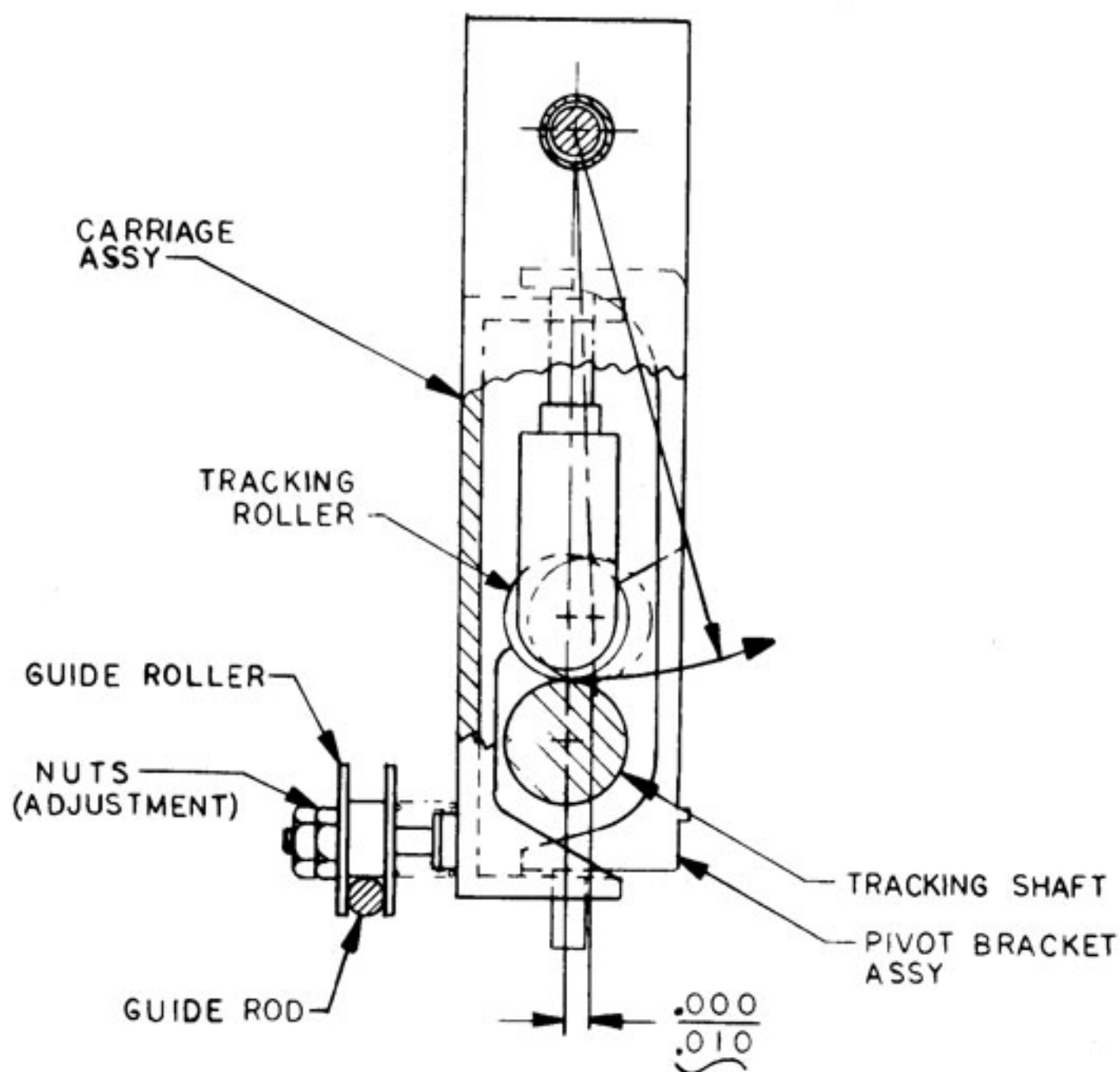
Figure 8. Carriage position adjustment
