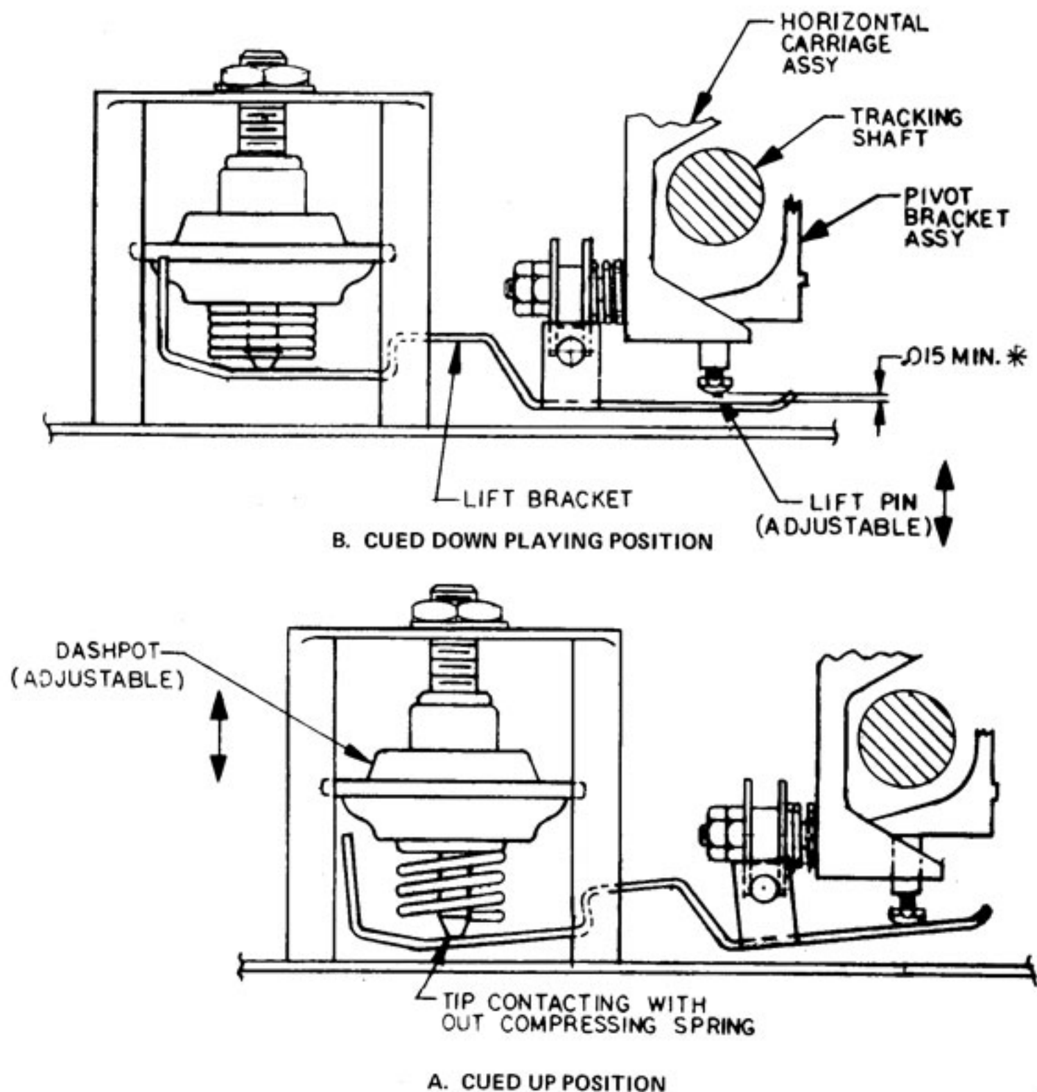
Figure 5. Tone arm lift adjustments
