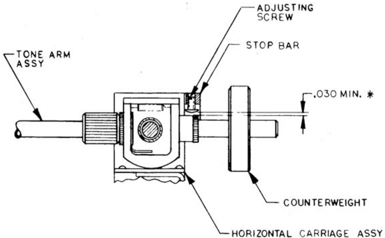
Figure 4. Tone arm cue lift adjustment
