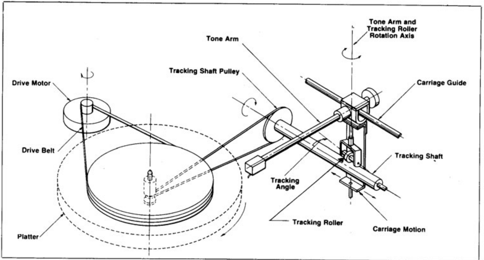
Figure 2. Tracking and drive schematic
