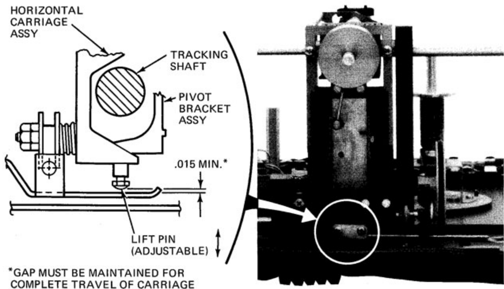
Figure 6. Threaded lift pin adjustment
