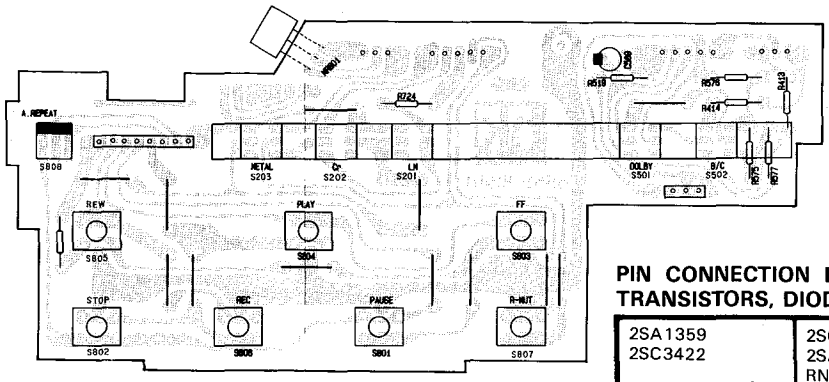
PCB-2 Function Switch P. C. Board
