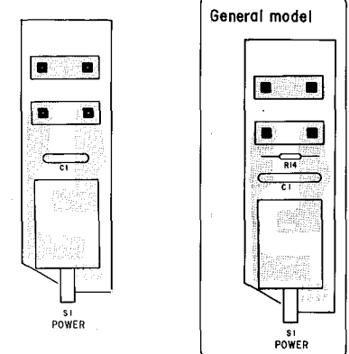
PCB-6 Dolby NR Ind. P. C. Board
