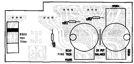
PCB-3 VR P. C. Board
