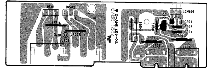
PCB-3 OUTPUT P. C. BOARD
