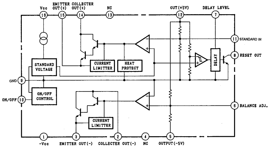
IC1: M5290P Voltage Regulator
