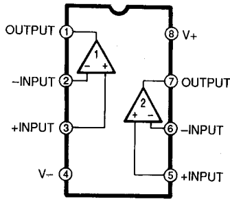
IC101, 501: NJM4565D OP-Amp., Headphones Amp.
