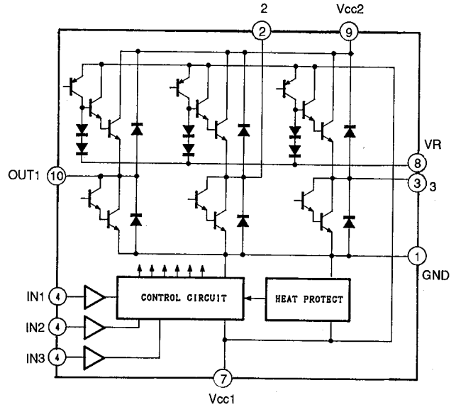
IC102: BA6247N Reversible Motor Driver
