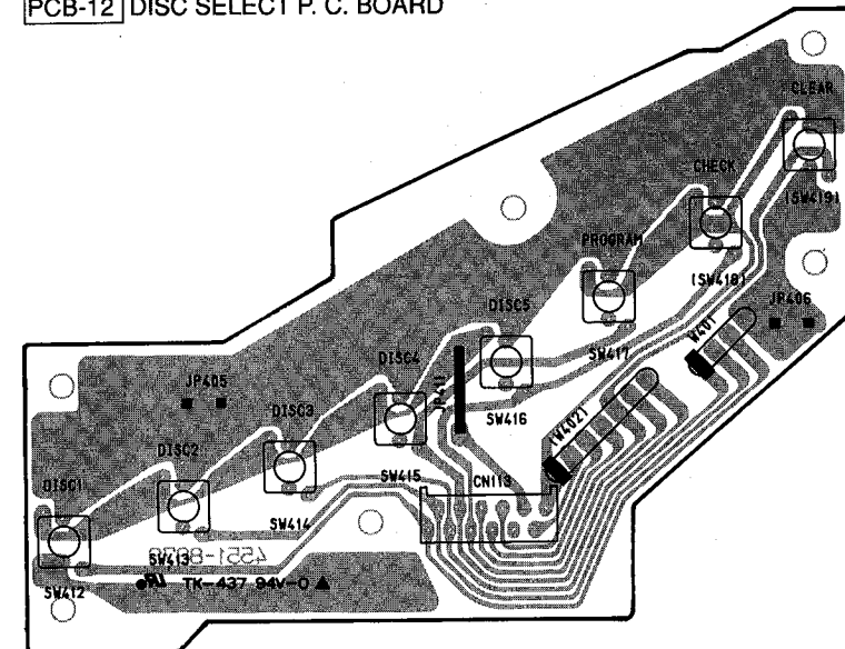
PCB-12 DISC SELECT P. C. BOARD
