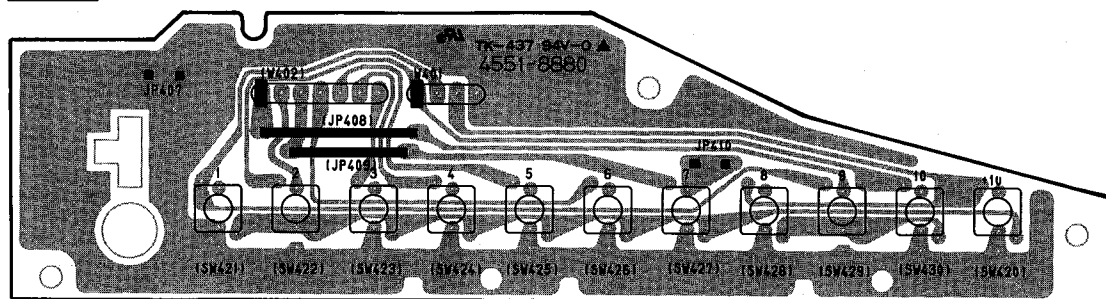
PCB-13 10 KEY P. C. BOARD
