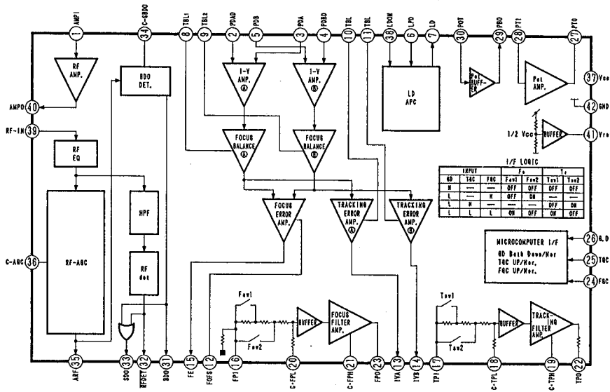
IC101: AN8373S Servo Amp.
