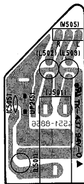
PCB-10 HEADPHONES P. C. BOARD
