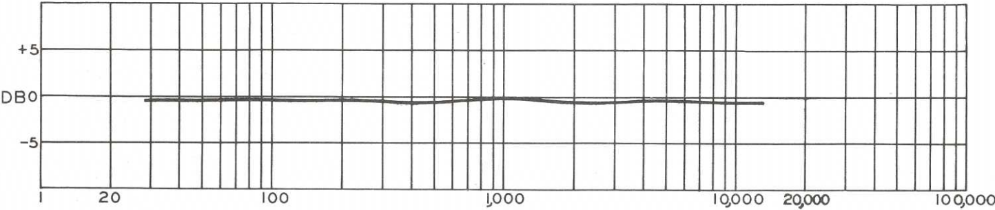
FREQUENCY RESPONSE AT 25 WATTS
