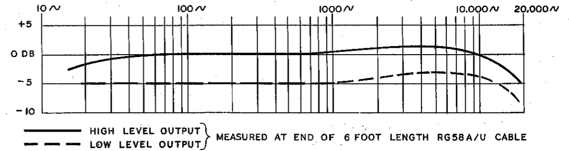
OVERALL CORRECTED FREQUENCY RESPONSE HEATHKIT FM-3A FM TUNER
