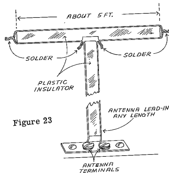
Figure 23 FOLDED DIPOLE ANTENNA MADE FROM 300 OHM TWIN- LEAD TRANSMISSION LINE
