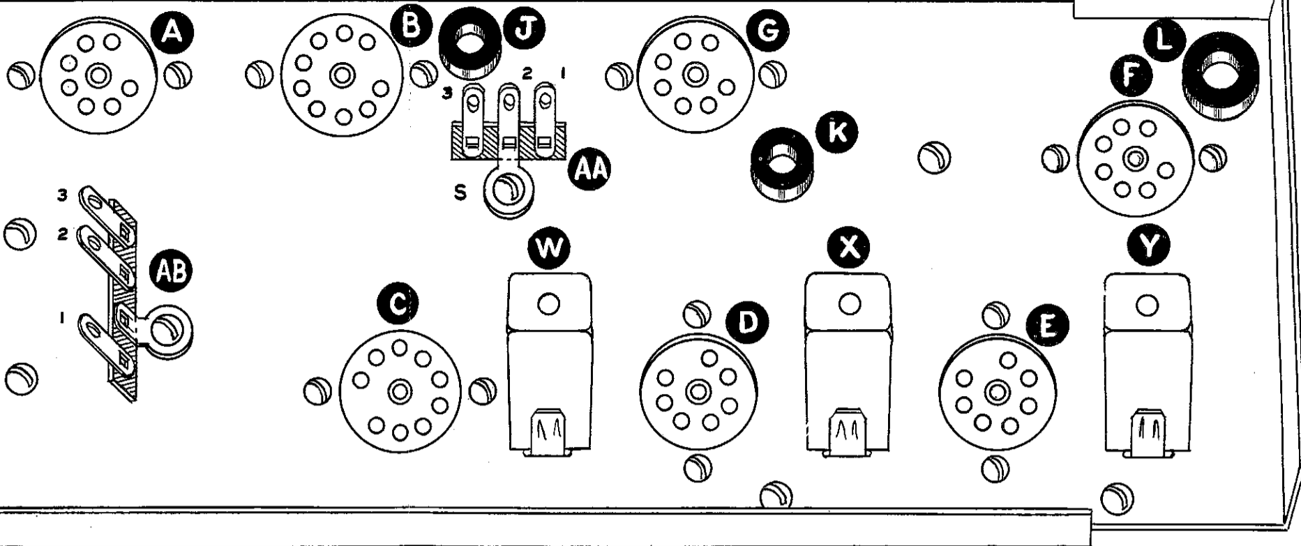
CHASSIS TOP
