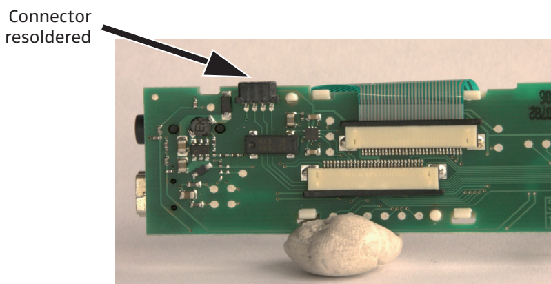
Figure 21: Connector re-attached
