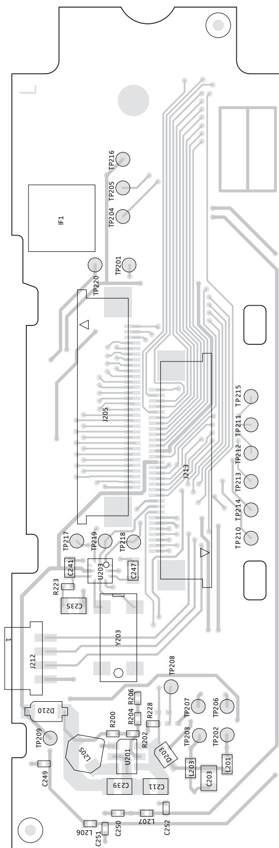
Connector board, printed circuit board, solder side
