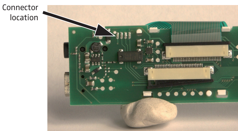
Figure 20: Connector location
