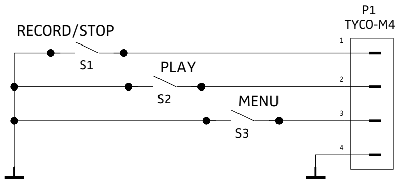
Keyboard PCB, circuit diagram
