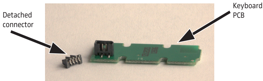
Figure 19: Keypad connector
