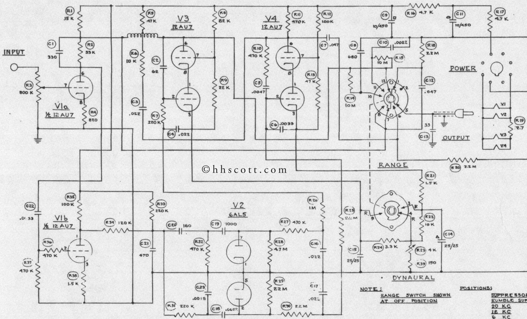
114-A DYNAURAL NOISE SUPPRESSOR CIRCUIT DIAGRAM
