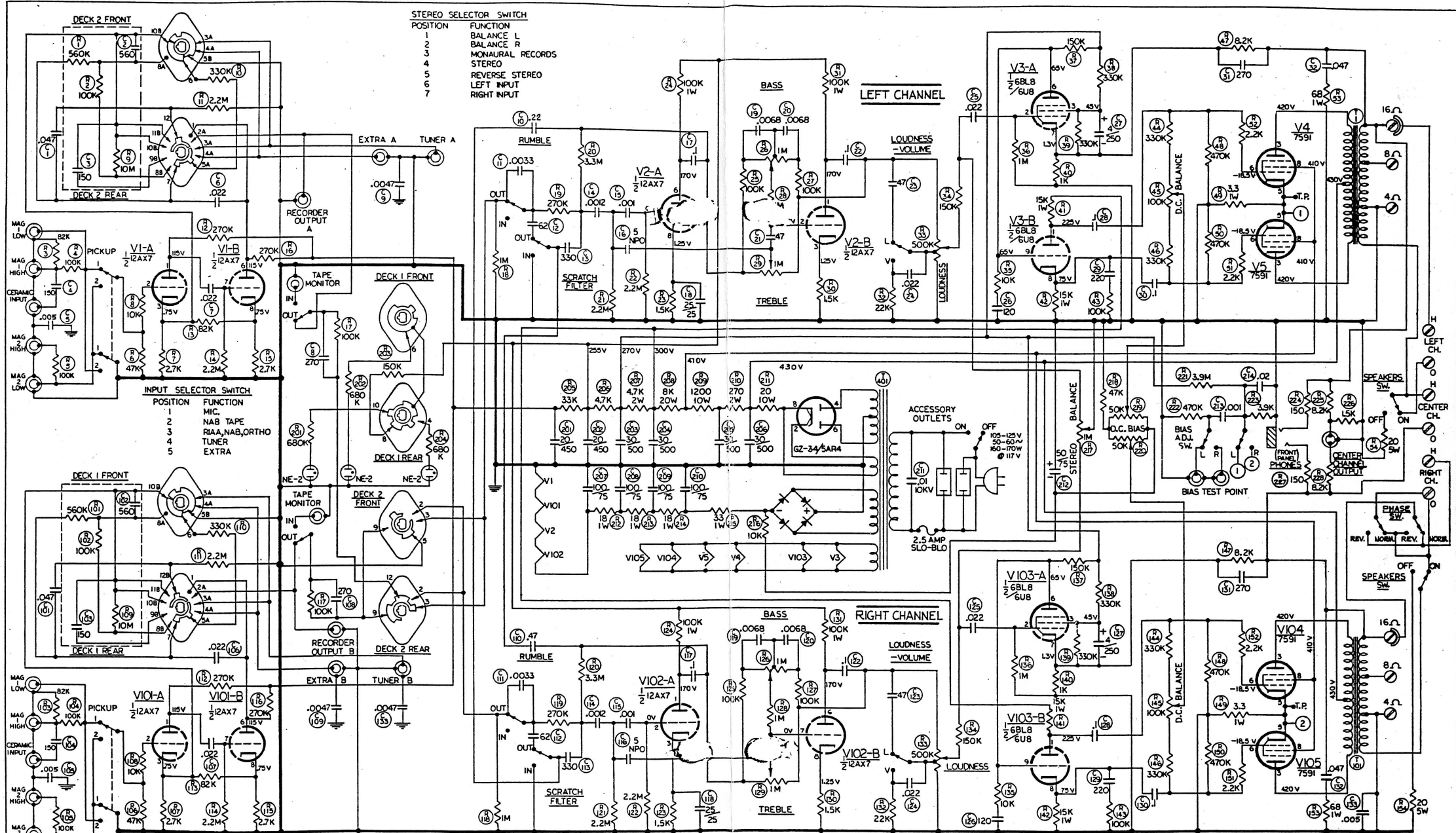
TYPE 299D STEREO AMPLIFIER
