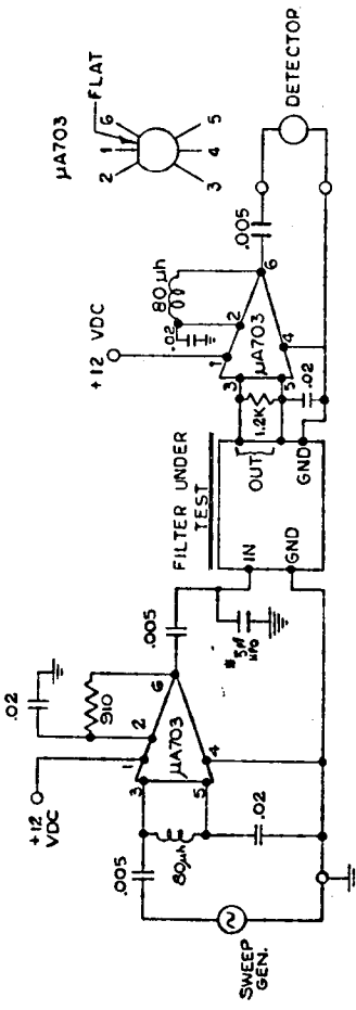
CRYSTAL FILTER TEST CIRCUIT
