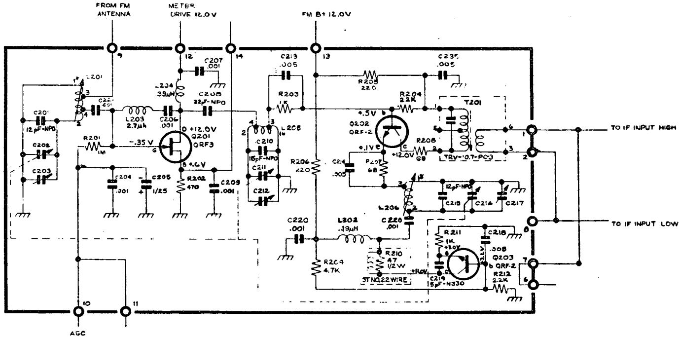
FM FRONT END
