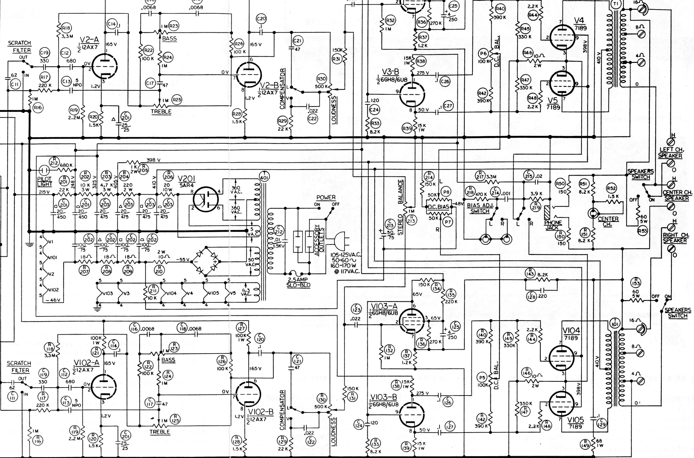
TYPE LK48B STEREO AMPLIFIER
