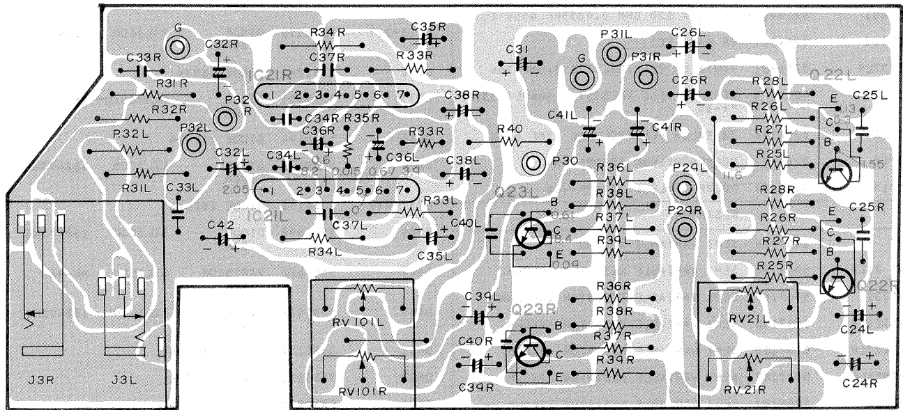
J 3 MIC RV 101 RECORD MIC RV 21 RECORD LINE
