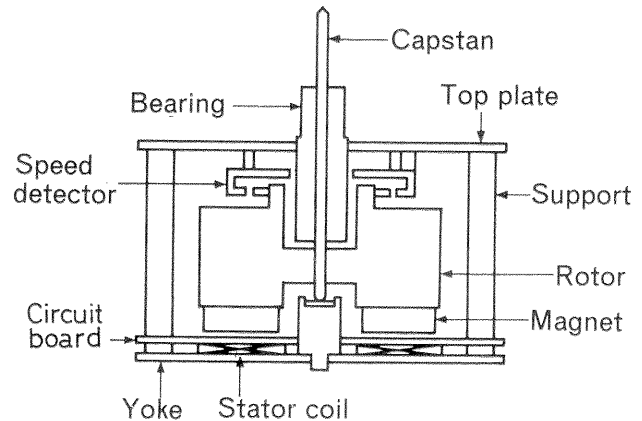
Fig. 19 Construction of three-phase uni-torque motor
