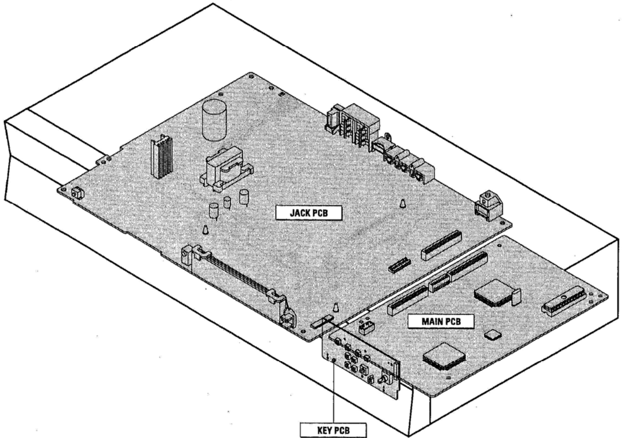
Fig. 4-6 PCB Location
