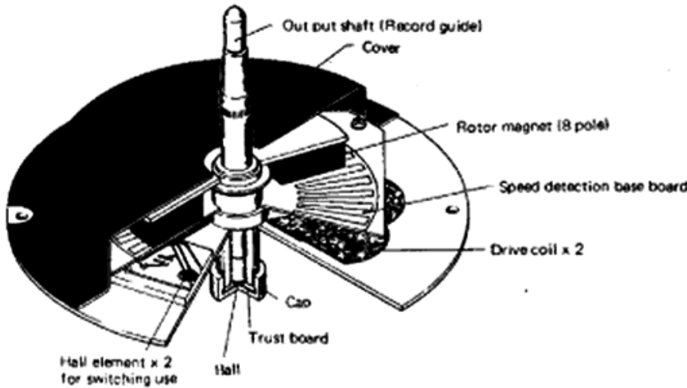
Fig. 2 Internal structure
