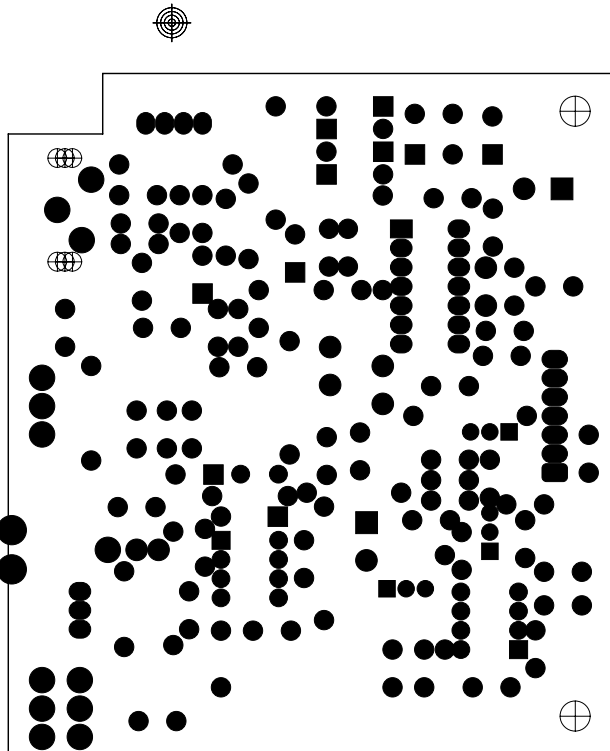
SOLDER MASK
