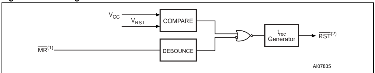
Figure 6. Block Diagram
