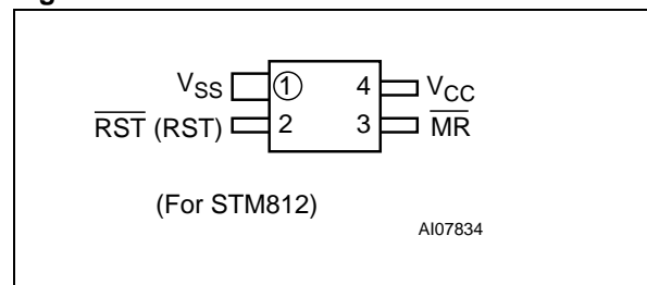
Figure 5. SOT143-4 Connections
