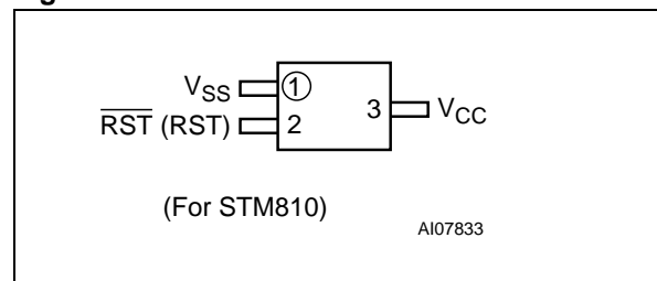
Figure 4. SOT23-3 Connections
