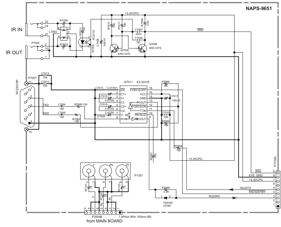
U13 RS-232C TERMINAL PC BOARD NAPS-9651
