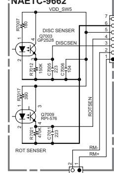
U12 DISC SENSOR PC BOARD NAETC-9662
