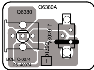
Soldering side view
