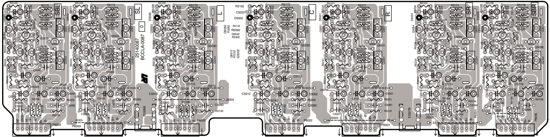
Soldering side view
