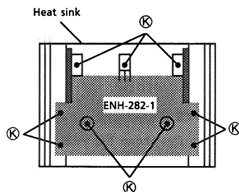
Fig-8. Heat sink ass'y
