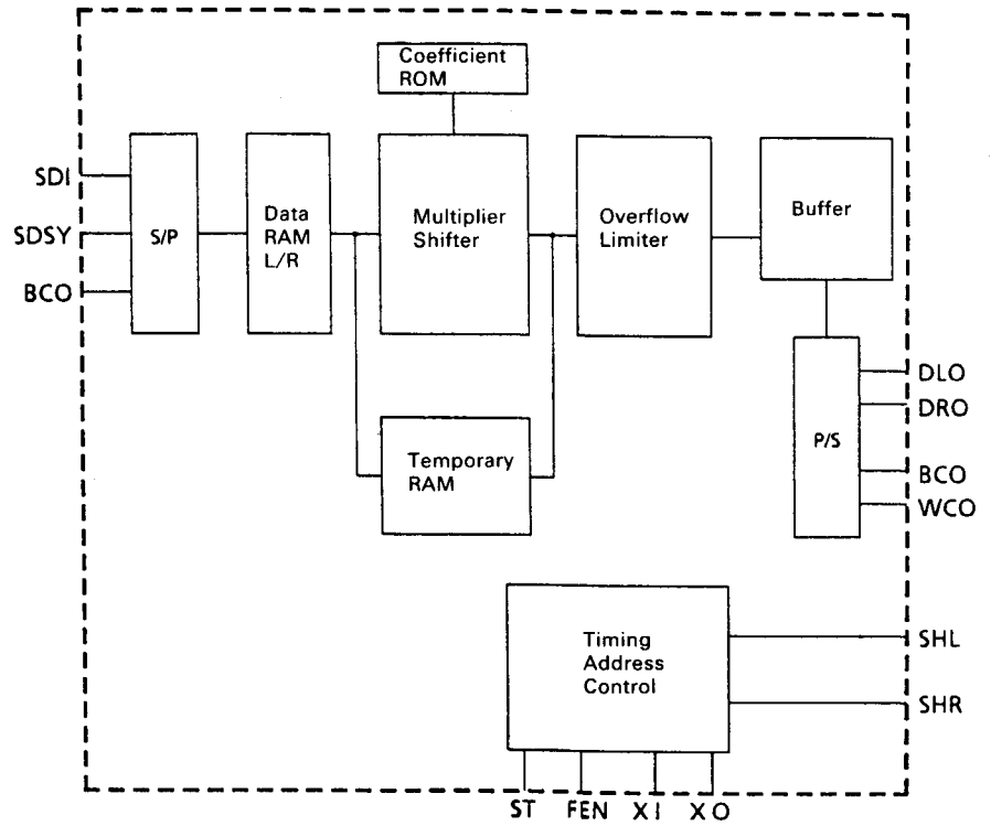
(2) Block Diagram
