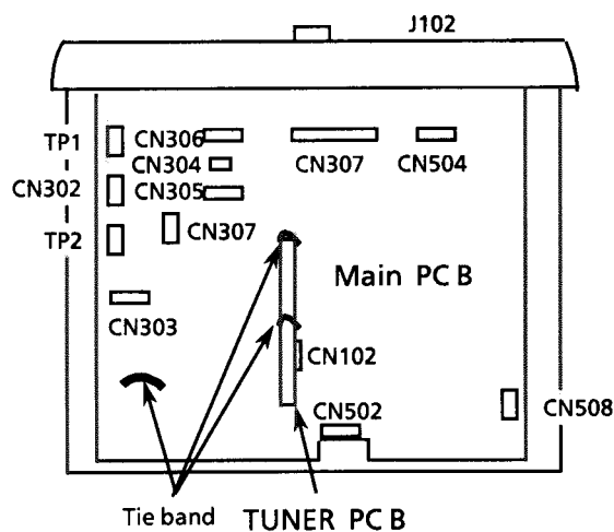
Fig3 Top view
