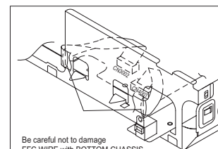
DRAWING FROM DIRECTION J FIG. 12
