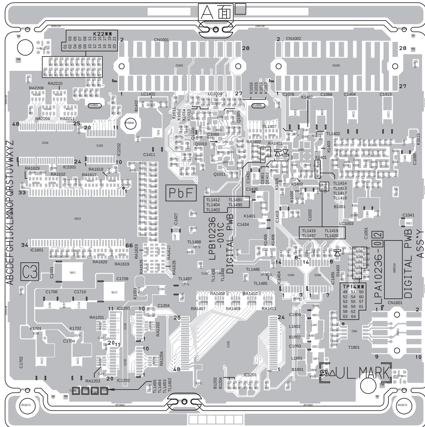
Forward side
