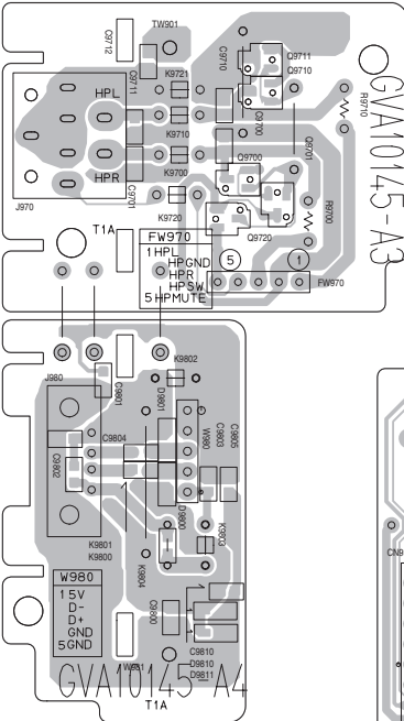
(USB board)
